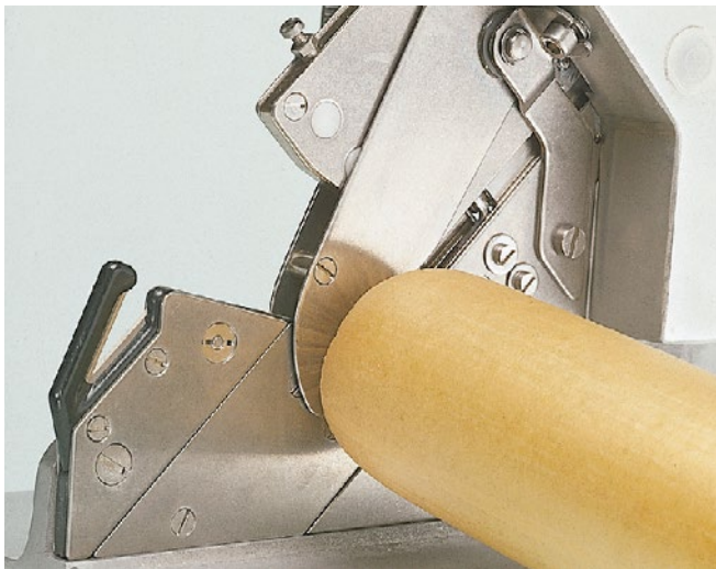
Excess casing or bag ends can be trimmed with the integrated cut-off knife.
