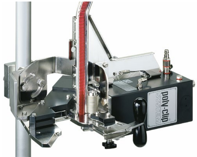
SCD 8100 as horizontal version
